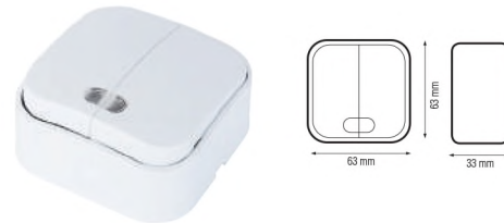
112 002 0002 ■ 2-GANG ILLUMINATED ONE WAY SWITCH (10A)
